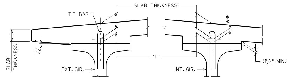
SLAB HAUNCH DETAIL
