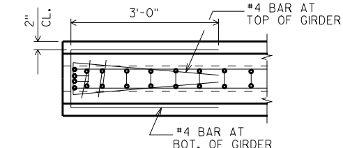
TOP VIEW OF GIRDER ENDS
