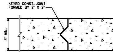
CONSTRUCTION JOINT
