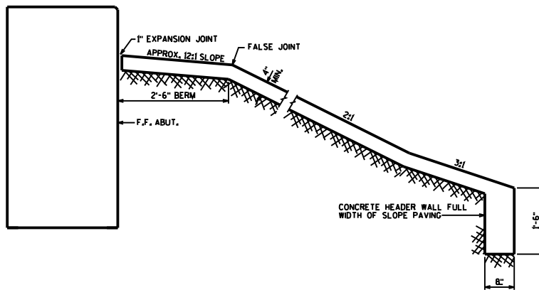
TYPICAL SECTION
