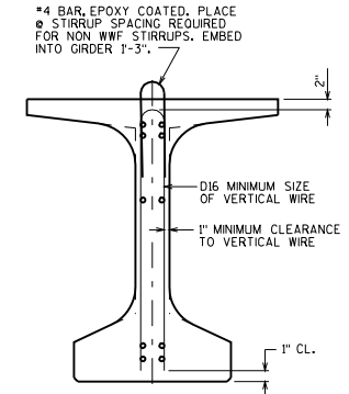
SECTION THRU GIRDER SHOWING WELDED WIRE FABRIC (WWF) STIRRUPS
