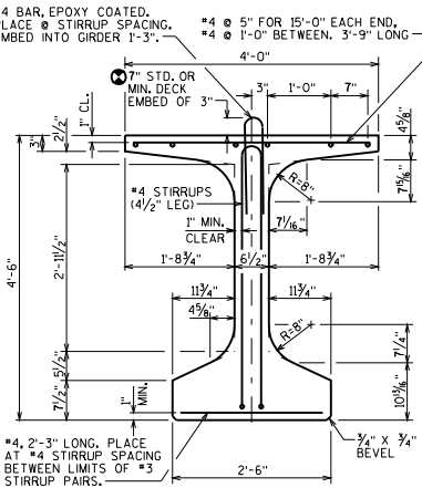
SECTION THRU GIRDER STRANDS NOT SHOWN
