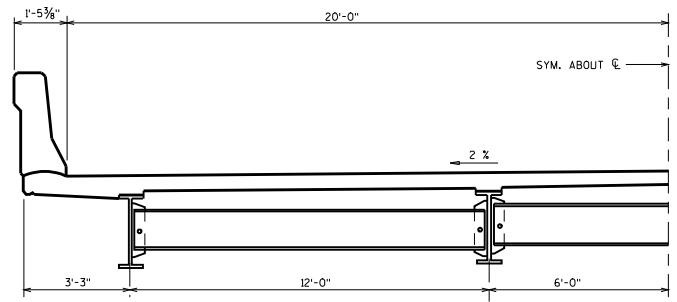
40'-0" ROADWAY
