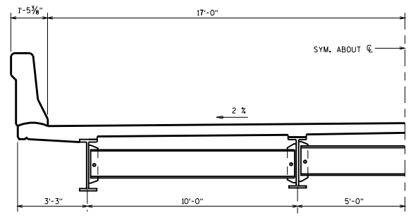
34'-0" ROADWAY
