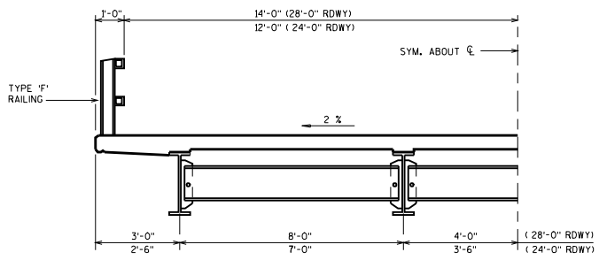
24'-0" & 28'-0" ROADWAY
