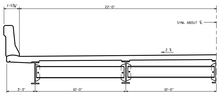
44'-0" ROADWAY
