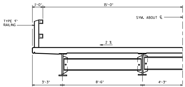
30'-0" ROADWAY
